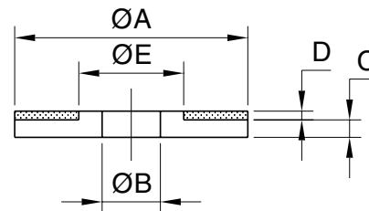
Type C Rebound Washer with Rubber
