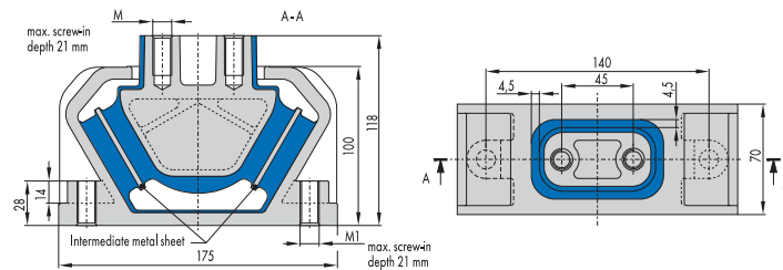
Fig. 4 Tapered Mounts 033 18 700, 033 18 701
